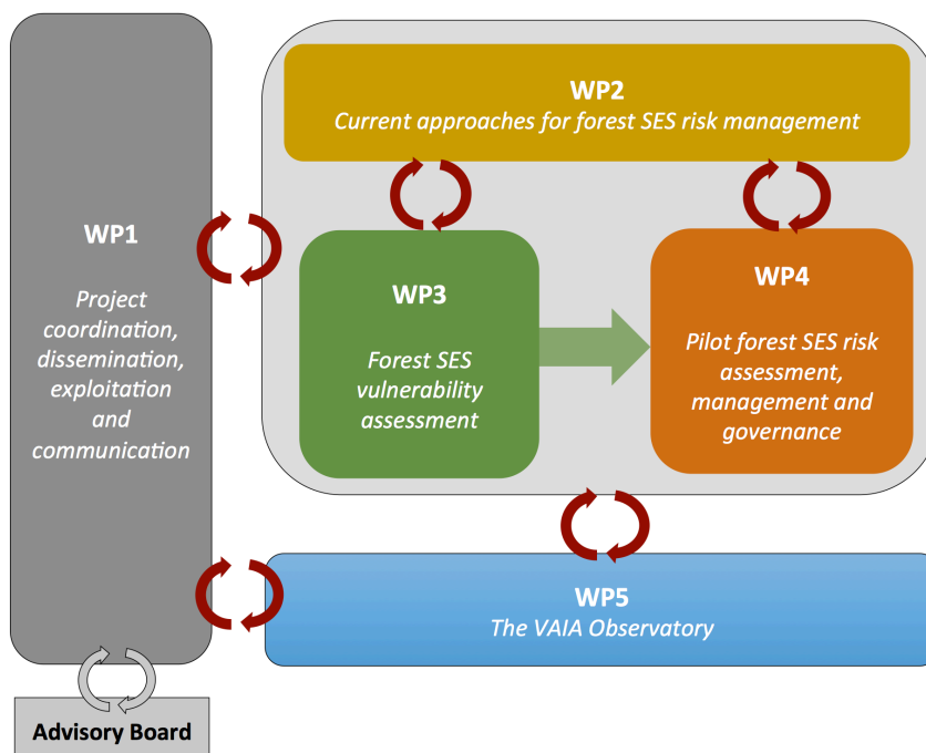
Fig.1 Project structure
